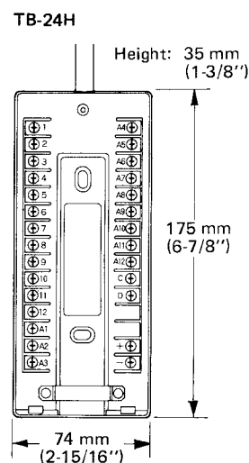
TERMINAL IDENTIFICATIONS
