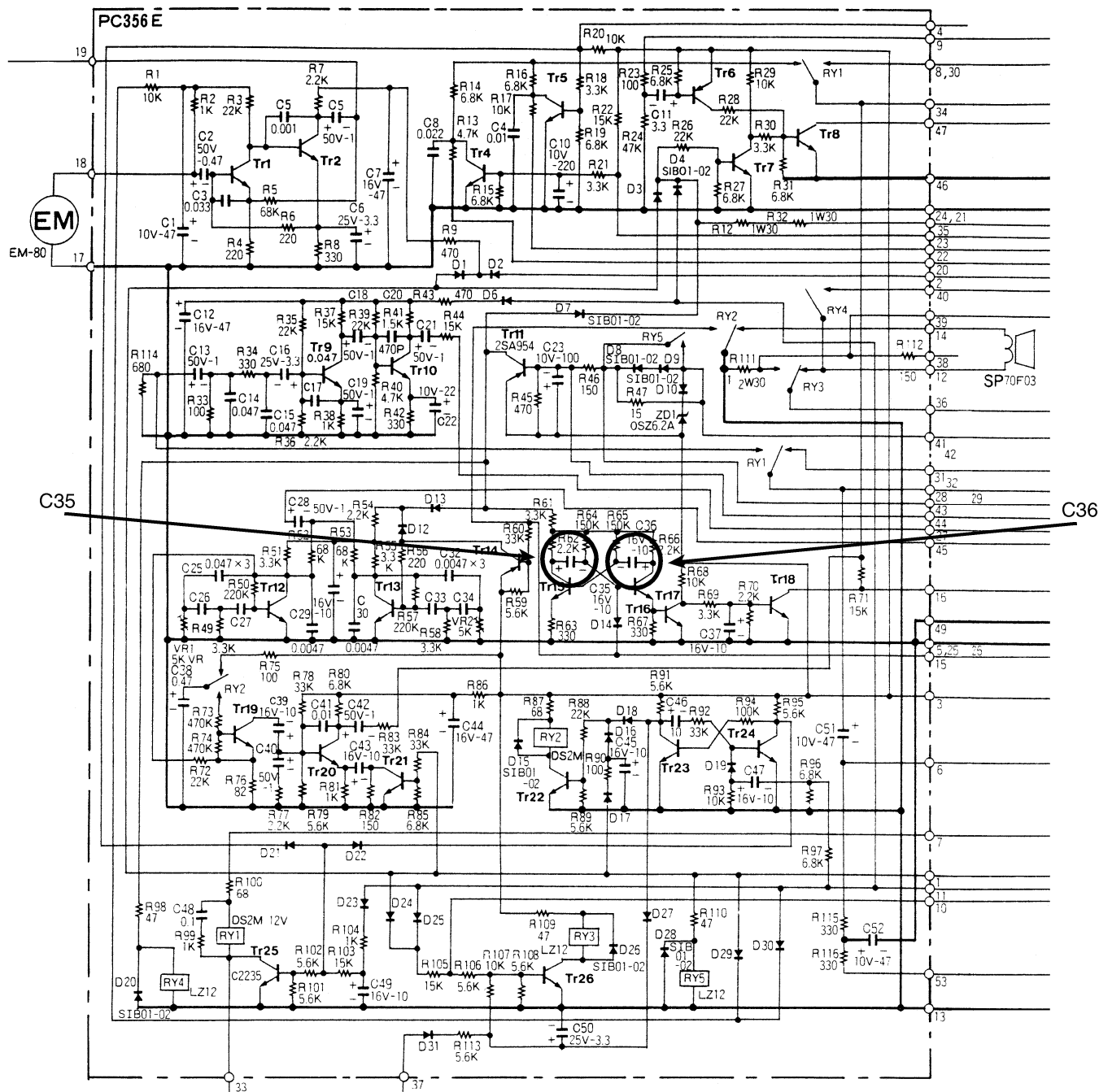
NEM Main PC Board Schematic Diagram
