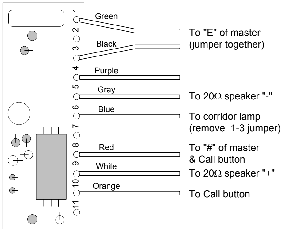
PC-454 (component view)
