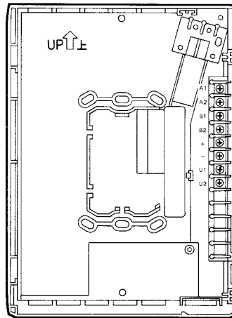
MYH-U CHASSIS INSIDE VIEW
